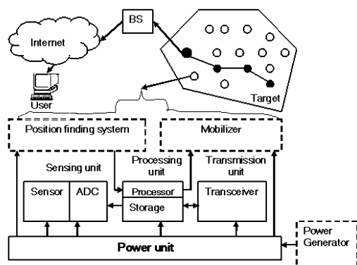
Figure 1: Structural view of sensor network
