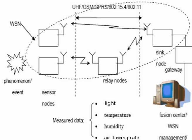
fig.6. EMS Prototype
