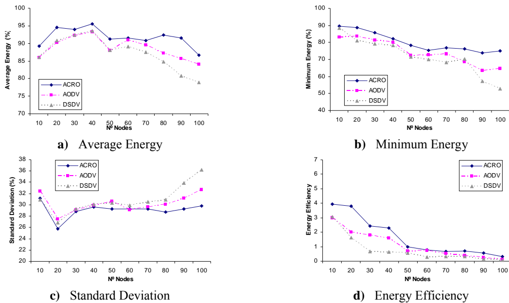
Figure 18: Energy performance comparison – moving phenomenon
