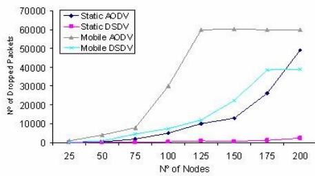
Figure 11: Dropped packets vs. network size
