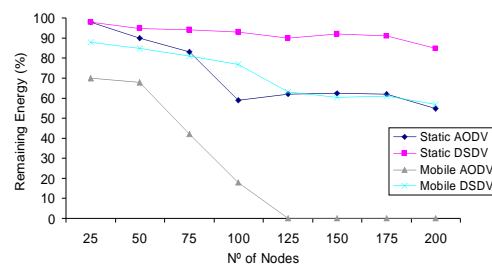
Figure 10: Remaining energy vs. network size
