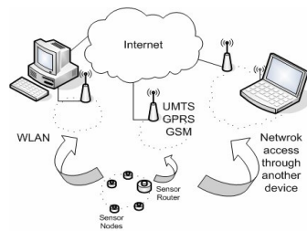
Figure 4: Connectivity model between IPSense and 4G networks
