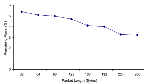
Figure 12: Remaining energy vs. packet length
