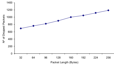
Figure 14: Dropped packets vs. packet length
