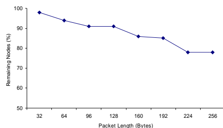
Figure 13: Remaining nodes vs. packet length
