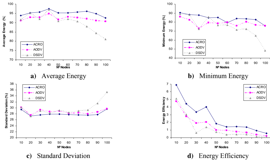
Figure 17: Energy performance comparison – static phenomenon
