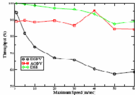
Fig.2 freeway throughput
