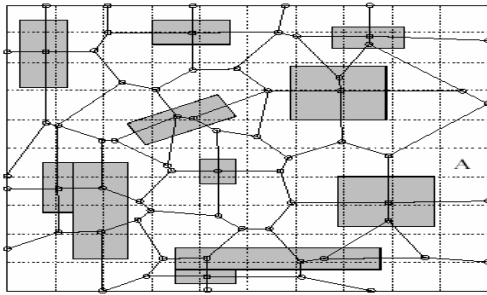
Fig.7 Voronoi Graph in simulation field
