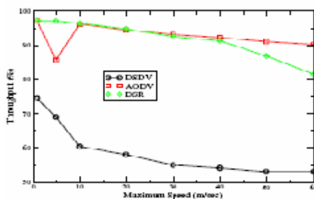
Fig.3 Manhattan throughput
