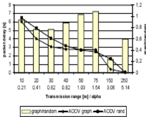
Fig.10 End-to-End Delay
