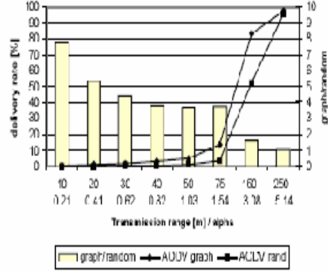
Fig.11 Packet Delivery Rate.
