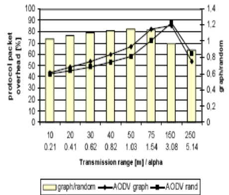
Fig.12 Data packet overhead
