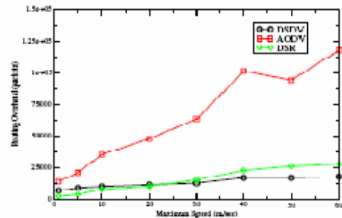
Fig.4 RWP Routing overhead
