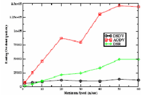
Fig.5 Freeway Routing overhead
