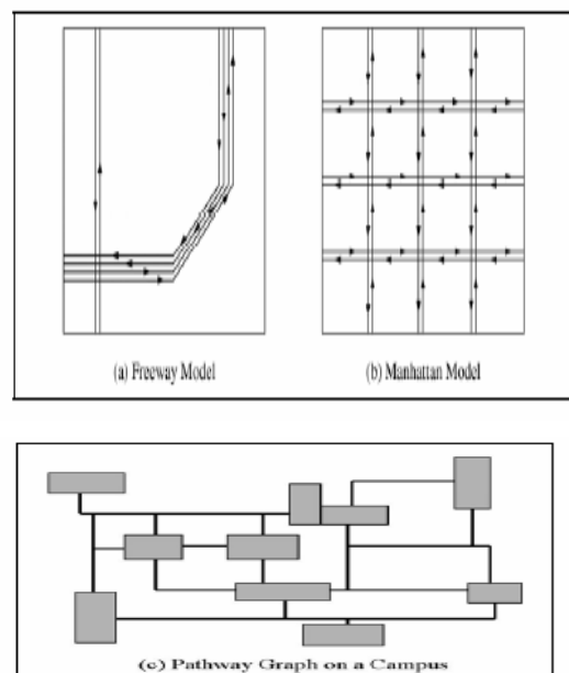
Fig. 3. The pathway graphs used in the Freeway, Manhattan and Pathway Model
