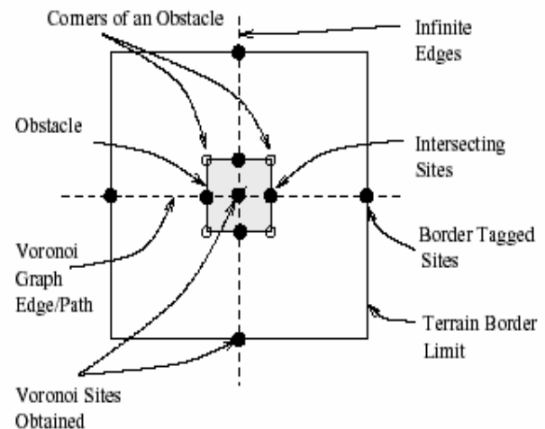
Fig. 5. Voronoi path and Obstacles
