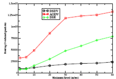
Fig.6 Manhattan Routing overhead
