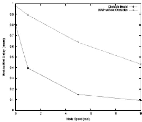
Fig.9 End-to-End Delay
