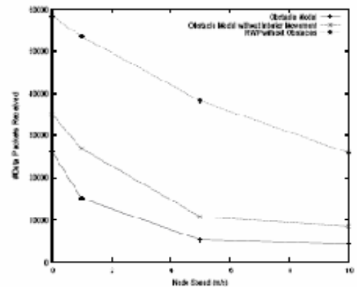
Fig.7 Data packet reception
